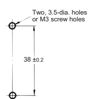
Mounting Hole Dimensions
