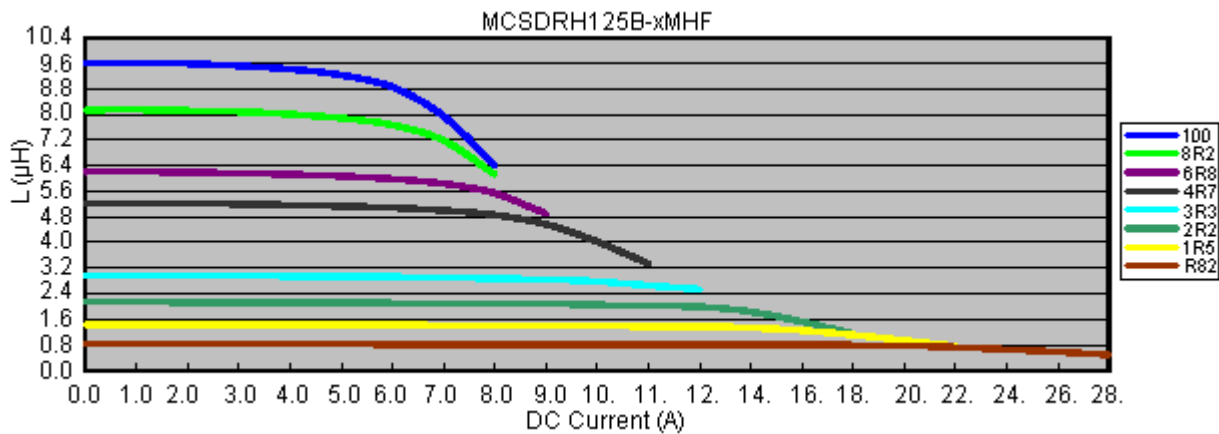
Inductance vs. Current
