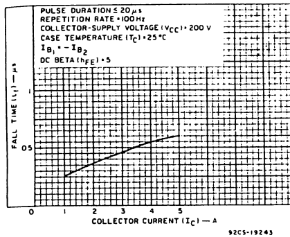
Fig. 11 - Typical fall-time vs. collector current for RCA431.
