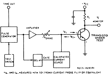
Fig. 16 - Circuit used to measure switching times.
