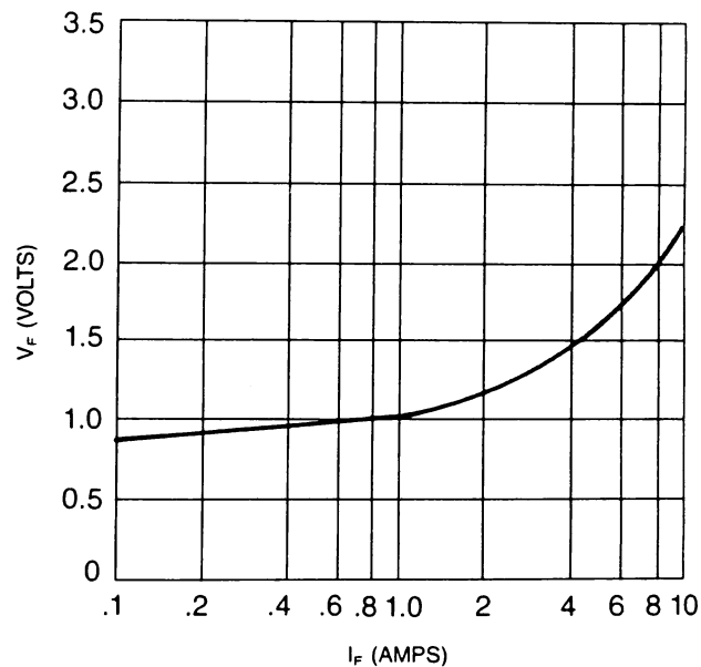
FORWARD VOLTAGE OF D1 (PMD 17K SERIES)
