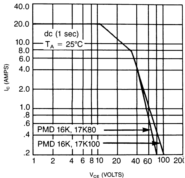
SAFE OPERATING AREA (PMD 16K, 17K SERIES)
