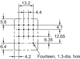
Mounting Hole and PCB Dimensions
