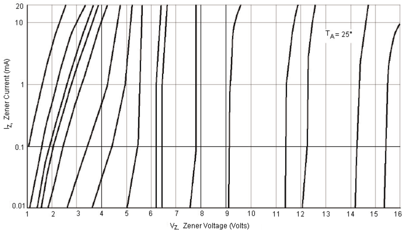
Zener Voltage versus Zener Current - V_Z = 1\text{ thru } 16\text{ Volts}
