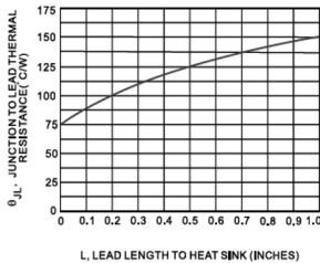
FIG. 3 - TYPICAL THERMAL RESISTANCE versus LEAD LENGTH
