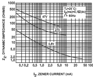
FIG. 6 - EFFECT OF ZENER CURRENT ON ZENER IMPEDANCE
