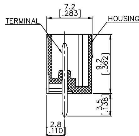
SECTION P-P
