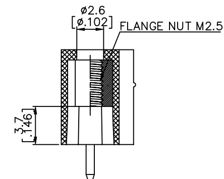
SECTION Q-Q
