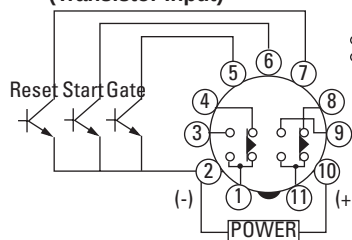
(Transistor Input)
