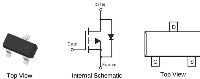
SOT23 (Standard)
