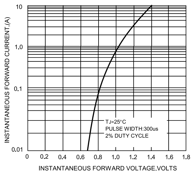
FIG.4-TYPICAL FORWARD CHARACTERISTICS
