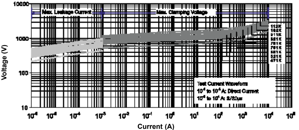
V-I Curve for SR471K to 112K14D(E) Series
