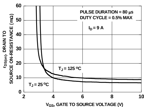
Figure 16. On-Resistance vs Gate to Source Voltage
