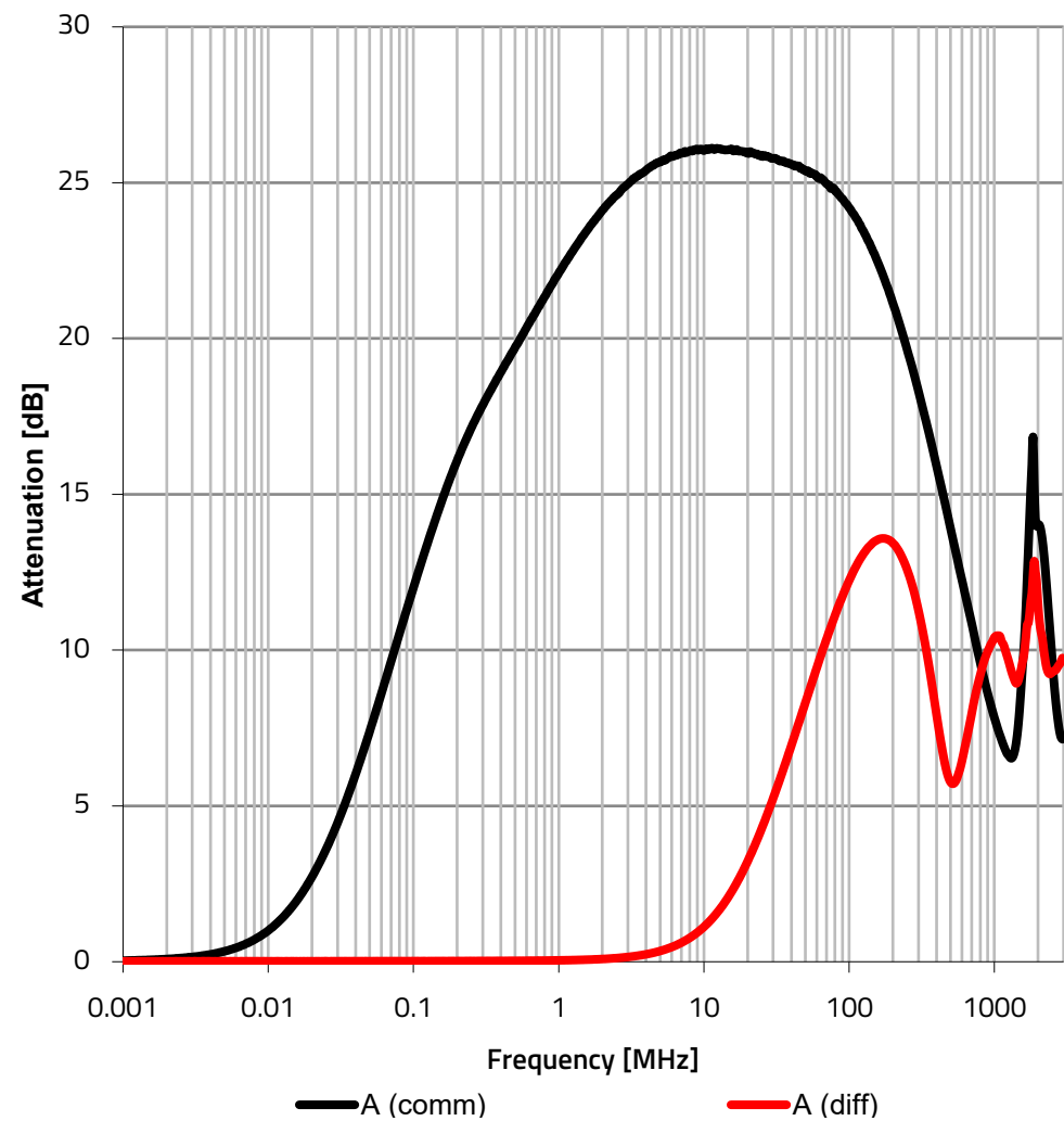
Typical Attenuation:
