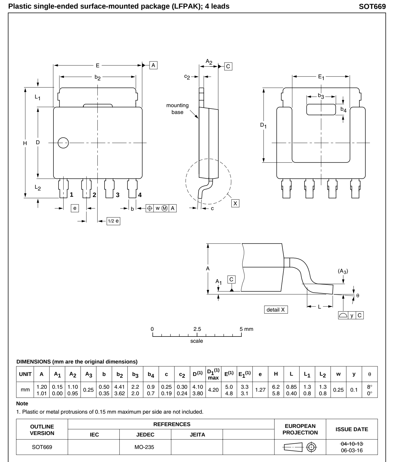
Fig 18. Package outline SOT669 (LPAK)
