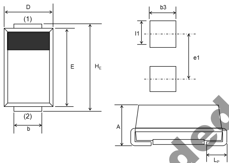
DO-214AC(SMA), (FVDS)
