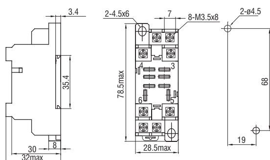
Mounting dimension
