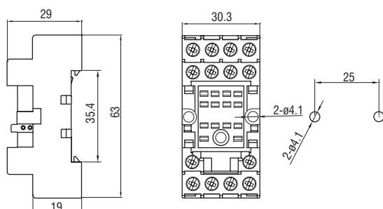
Mounting dimension
