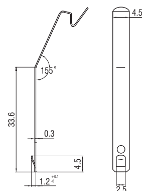
Retainer dimension
