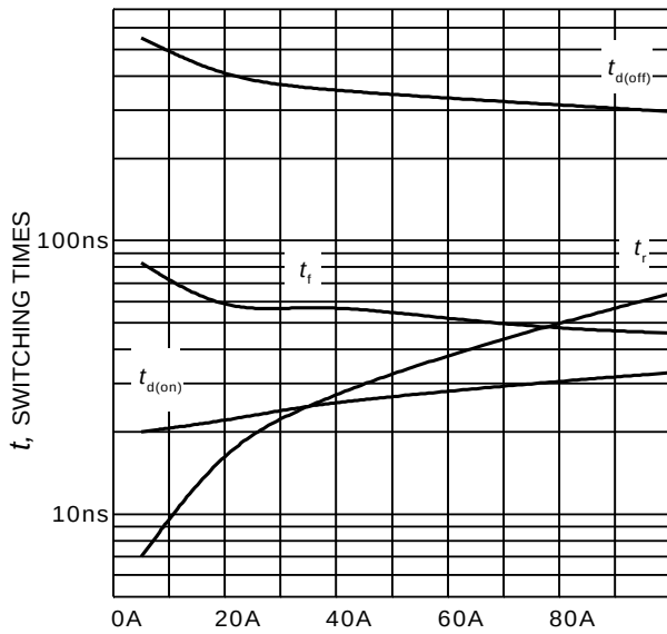
Figure 9. Typical switching times as a function of collector current (inductive load, T J =175°C, V CE = 400V, V GE = 0/15V, r G = 7Ω, Dynamic test circuit in Figure E)
