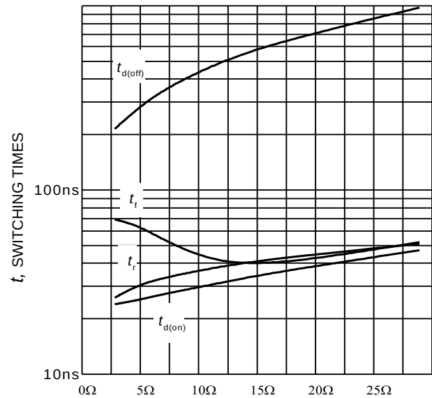
Figure 10. Typical switching times as a function of gate resistor (inductive load, T J = 175°C, V CE = 400V, V GE = 0/15V, I C = 50A, Dynamic test circuit in Figure E)
