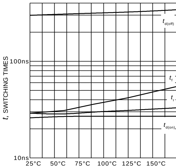
Figure 11. Typical switching times as a function of junction temperature (inductive load, V CE = 400V, V GE = 0/15V, I C = 50A, r G =7Ω, Dynamic test circuit in Figure E)
