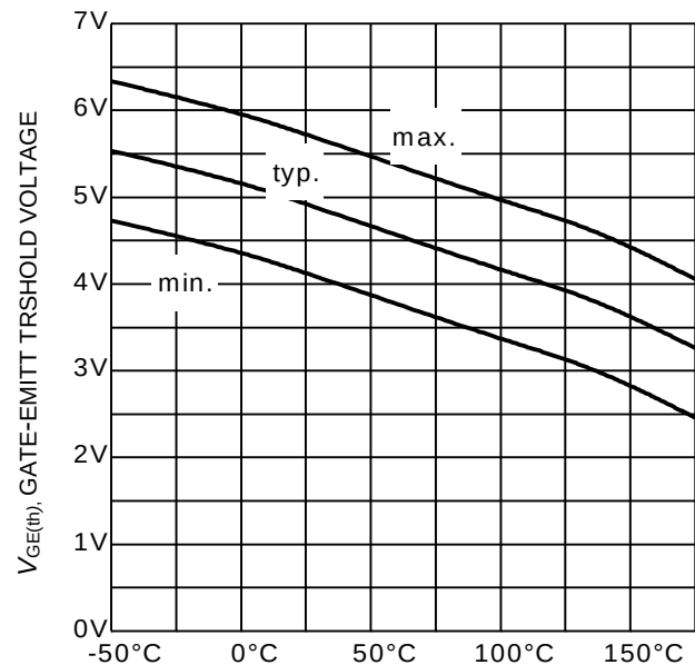
Figure 12. Gate-emitter threshold voltage as a function of junction temperature (I C = 0.8mA)
