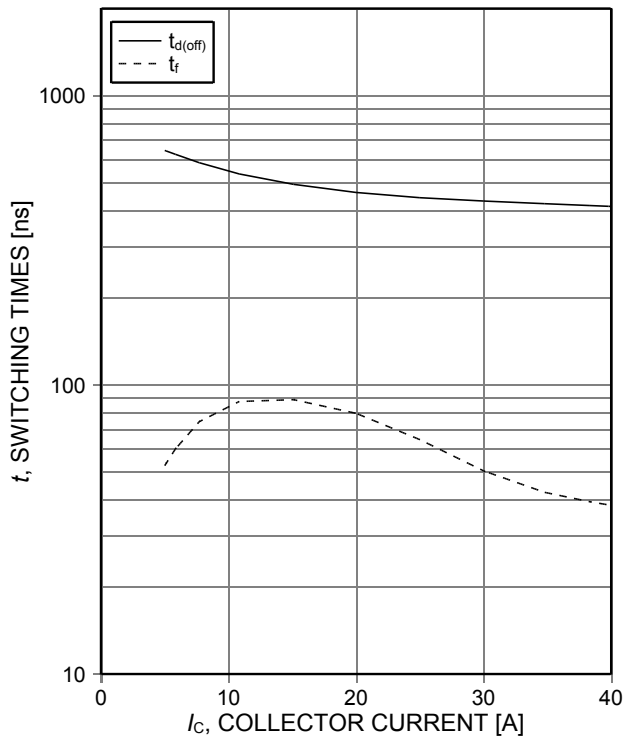
Figure 9. Typical switching times as a function of collector current (ind. load, T_J=175^{\circ}\text{C} , V_{CE}=600\text{V} , V_{GE}=0/15\text{V} , R_{G(on)}=15\Omega , R_{G(off)}=15\Omega , test circuit in Fig. E)
