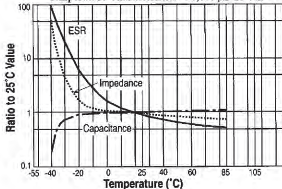
Temperature Characteristics - 98,000 \mu F 10 Vdc
