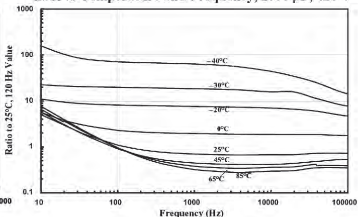
ESR vs Temperature and Frequency, 2700 \mu F, 420 V
