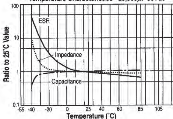
Temperature Characteristics - 29,000 \mu F 50Vdc
