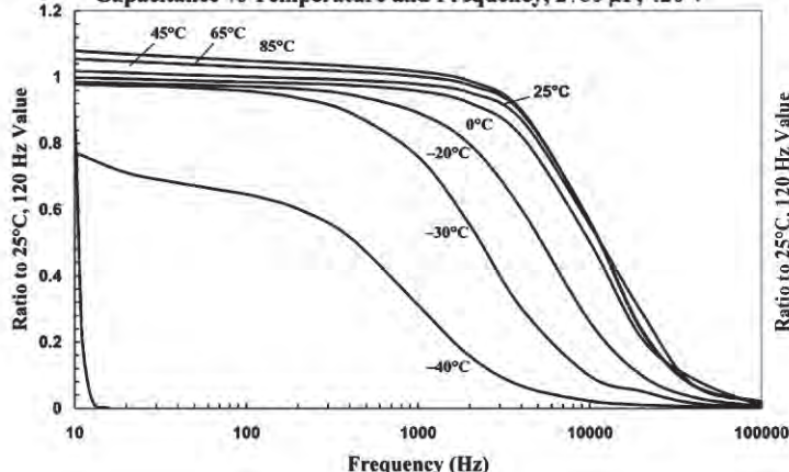
Capacitance vs Temperature and Frequency, 2700 \mu F, 420 V
