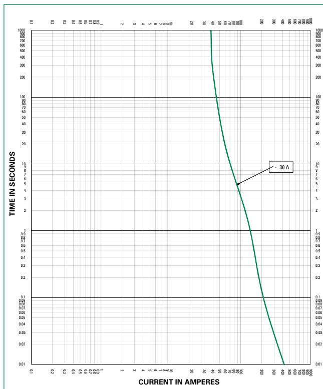
Time Current Curve (30 A)
