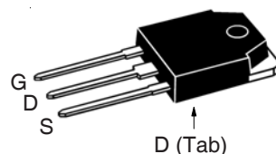
TO-247 (IXTH)
