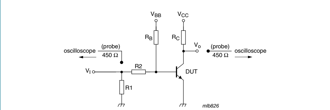
Fig 14. Test circuit for switching times
