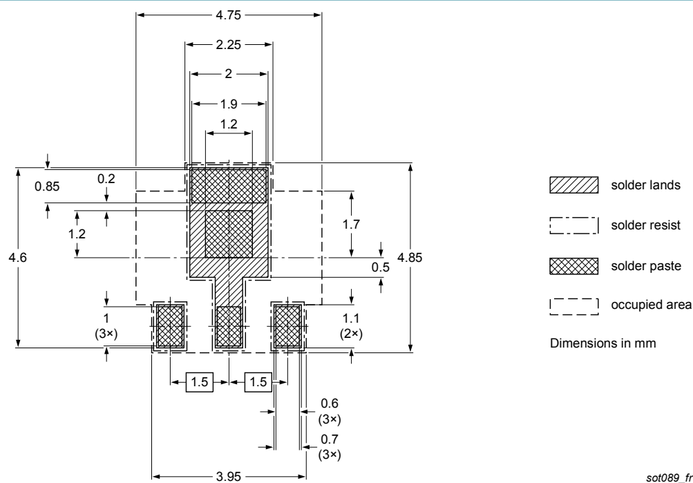
Fig. 16. Reflow soldering footprint for SOT89
