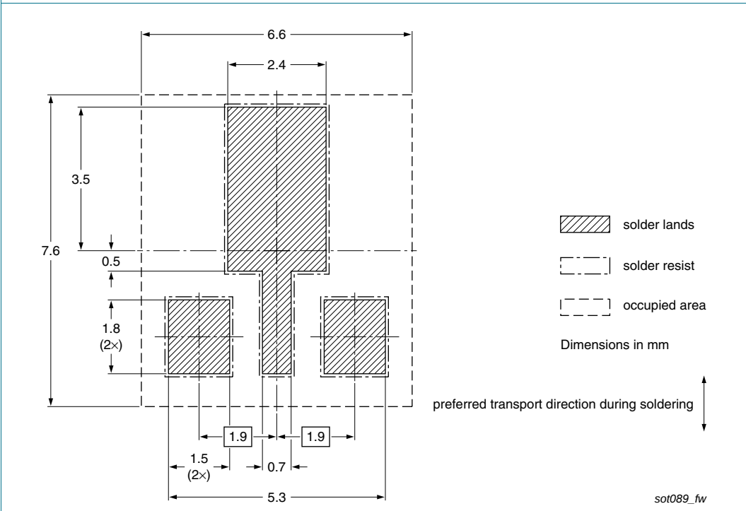
Fig 15. Wave soldering footprint SOT89 (SC-62/TO-243)
