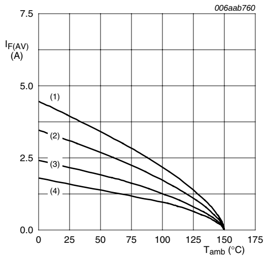
FR4 PCB, standard footprint T_j = 150^\circ\text{C} (1) \delta = 1 ; DC (2) \delta = 0.5 ; f = 20\text{ kHz} (3) \delta = 0.2 ; f = 20\text{ kHz} (4) \delta = 0.1 ; f = 20\text{ kHz}
