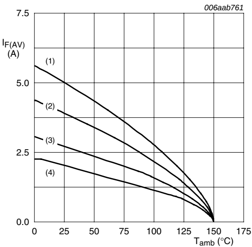
FR4 PCB, mounting pad for cathode 1\text{ cm}^2 T_j = 150^\circ\text{C} (1) \delta = 1 ; DC (2) \delta = 0.5 ; f = 20\text{ kHz} (3) \delta = 0.2 ; f = 20\text{ kHz} (4) \delta = 0.1 ; f = 20\text{ kHz}
