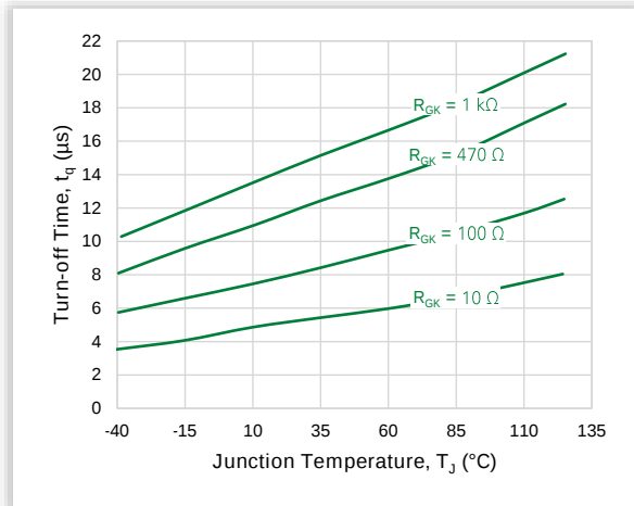
Figure 13. Typical DC Turn-off Time with R_{GK} vs. Junction Temperature for S6X8xS
