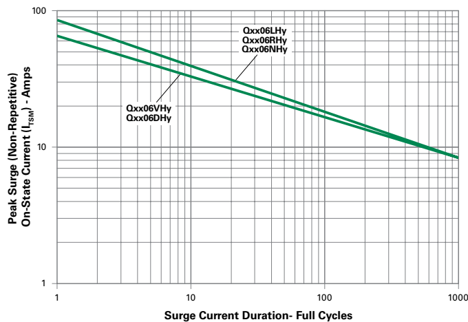
Figure 13: Surge Peak On-State Current vs. Number of Cycles (Alternistor Triac)
