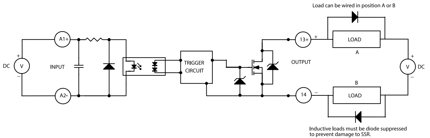
BLOCK DIAGRAM, CN100DXX,CN024DXX DC CONTROL - DC OUTPUT
