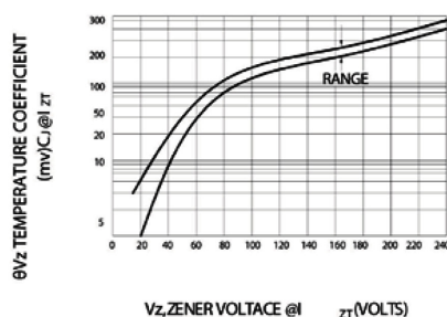
FIG.2 - TEMPERATURE COEFFICIENT RANGE
