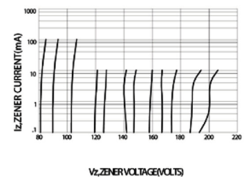
FIG.9 – ZENER VOLTAGE VERSUS ZENER CURRENT V_Z = 82 \text{ THRU } 200 \text{ VOLTS}
