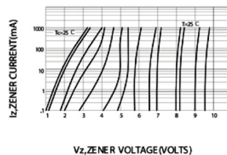
FIG.7 – ZENER VOLTAGE VERSUS ZENER CURRENT Vz=6.8 THRU 10 VOLTS
