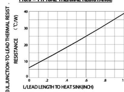
FIG.3 - TYPICAL THERMAL RESISTANCE
