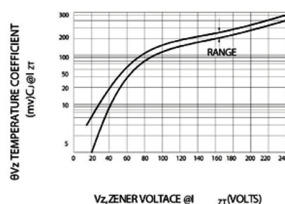
FIG.2 - TEMPERATURE COEFFICIENT RANGE
