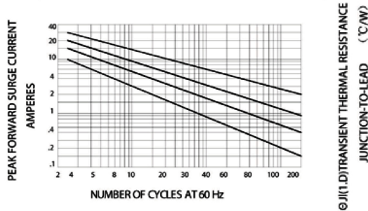
FIG.4 – MAXIMUM NON-REPETITIVE SURGE CURRENT
