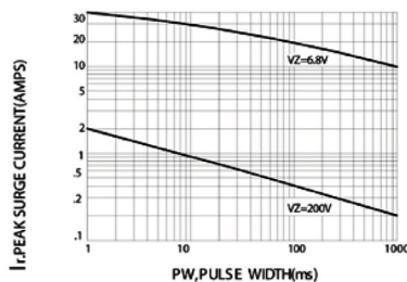
FIG.6 – PEAK SURGE CURRENT VERSUS PULSE WIDTH
