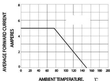
FIG.1 -FORWARD DERATING CURVE
