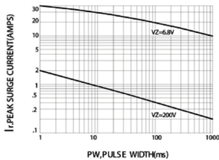
FIG.6 – PEAK SURGE CURRENT VERSUS PULSE WIDTH
