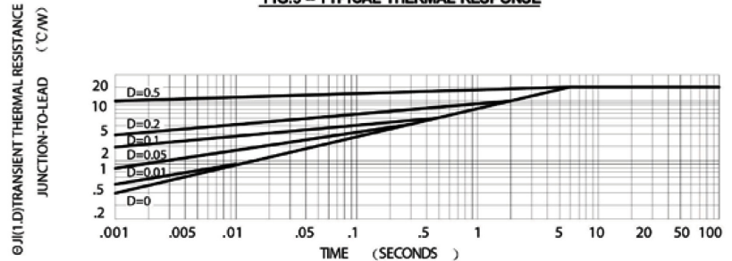
FIG.5 – TYPICAL THERMAL RESPONSE
