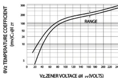
FIG.2 – TEMPERATURE COEFFICIENT RANGE
