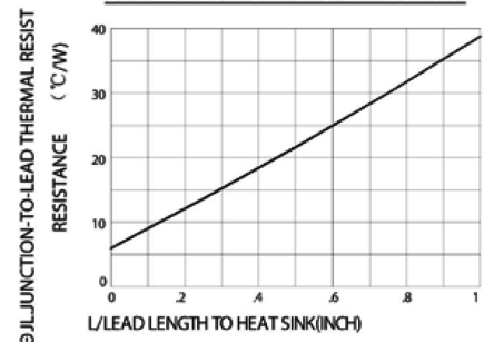
FIG.3 – TYPICAL THERMAL RESISTANCE
