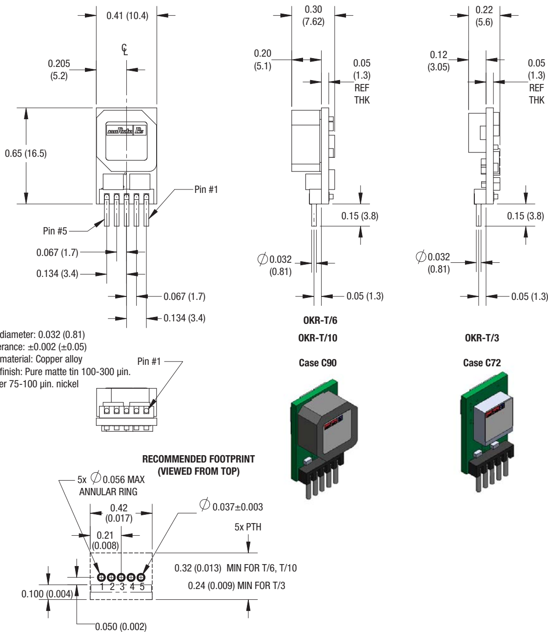
Figure 2. OKR Series Component locations are typical.
