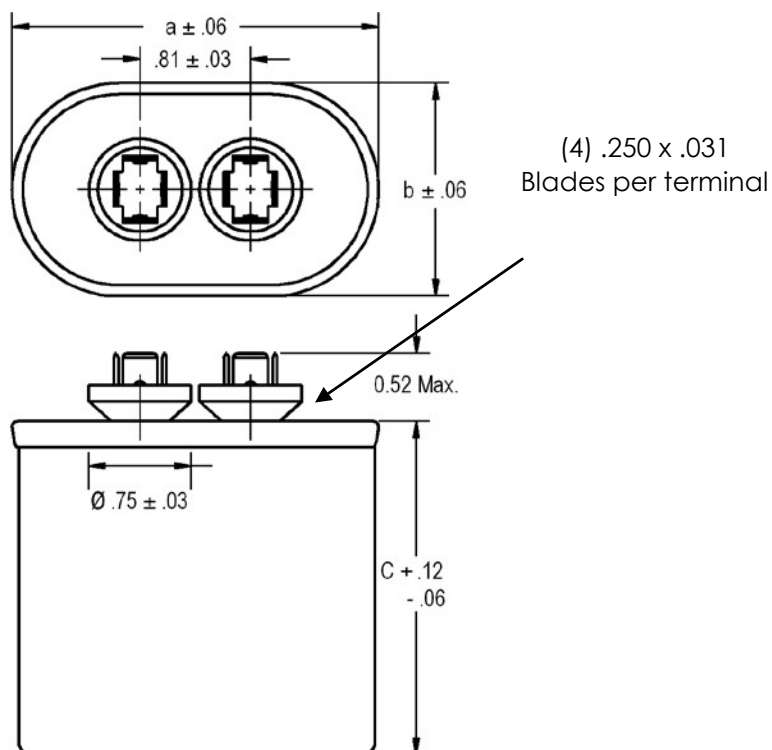
Case Style A,B,C,D
