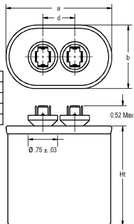
GEM III (27L Series) Outline
