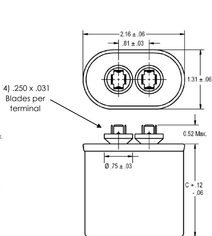
Case Style A
