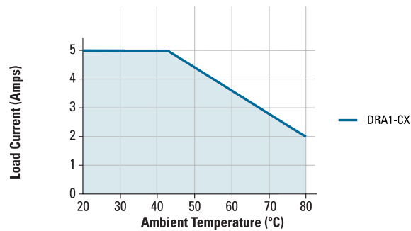
DRA1-CX Derating Curve
