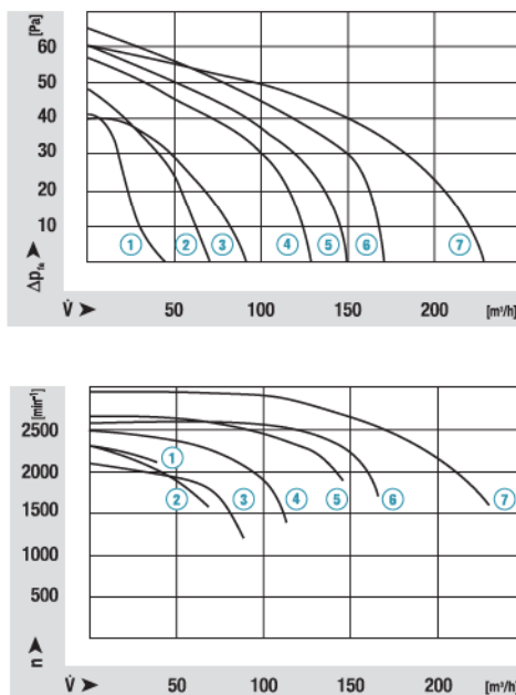
Characteristic curves
