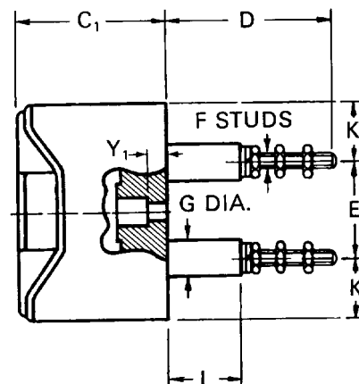
BACK CONNECTED — SURFACE
