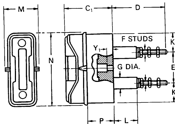
BACK CONNECTED — FLUSH
