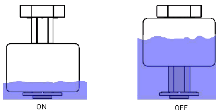
Operating Diagram
