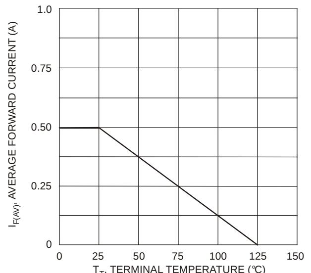
Fig. 4 Forward Current Derating Curve
