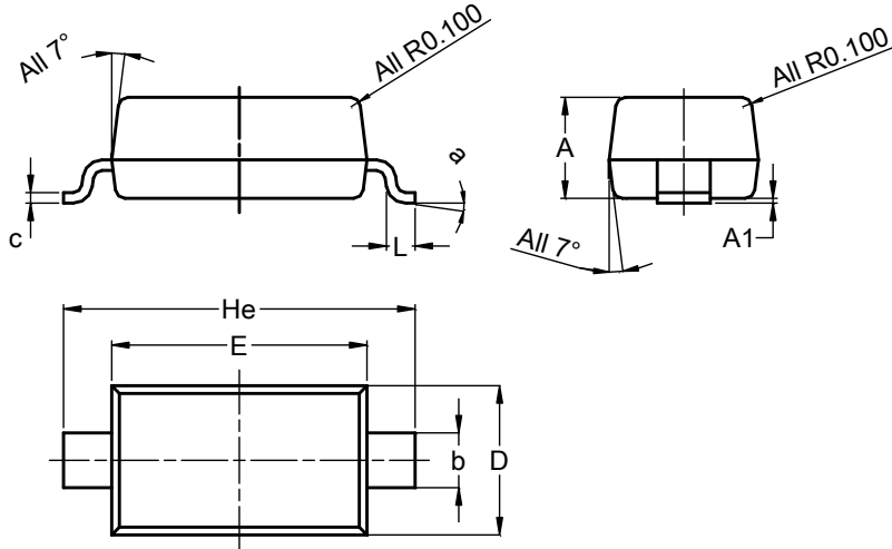
SOD123
