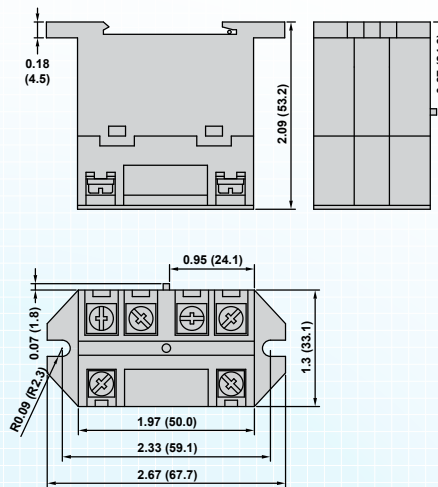
C3 – PANEL/DIN MOUNT (SCREW TERMINAL)
