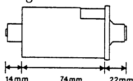
Panel mounting version
