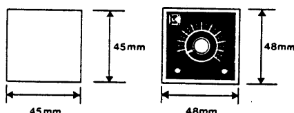
Cut-out dimensions
