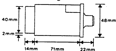
Panel mounting version
