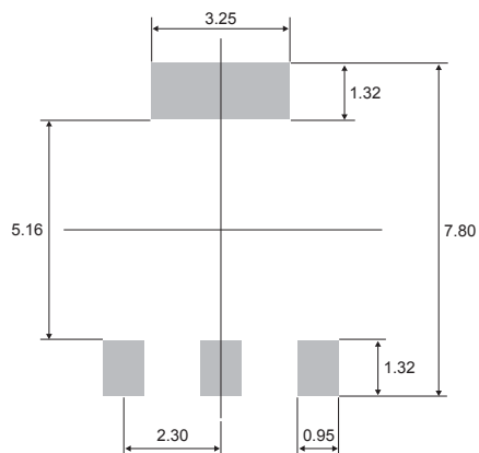
Figure 17. SOT-223 footprint (dimensions in mm)
