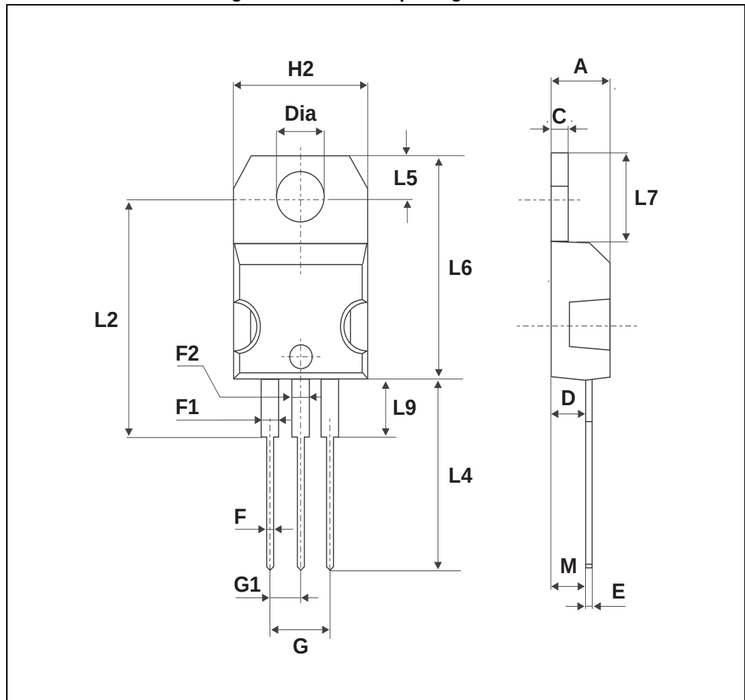
Figure 17. TO-220AB package outline
