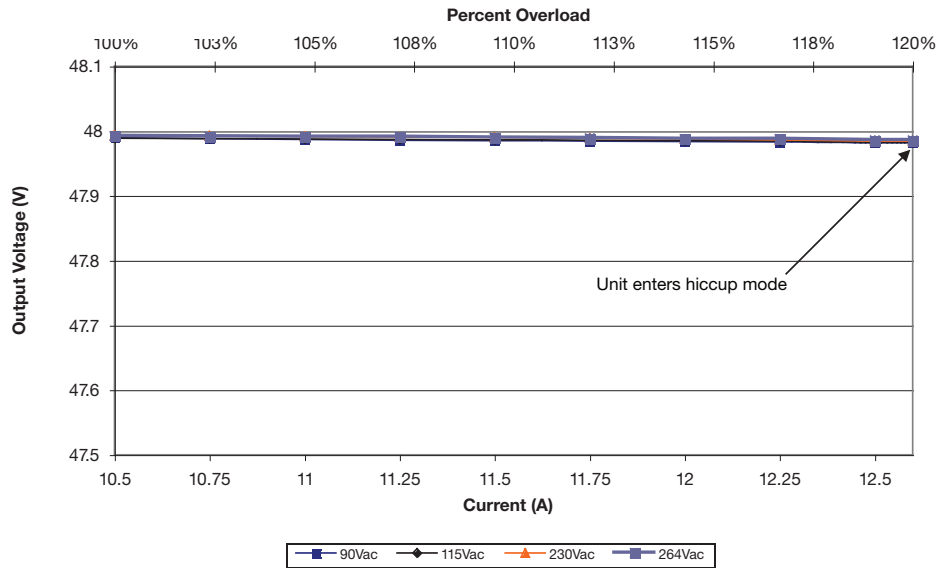
Figure 3 - LCL500PS48
