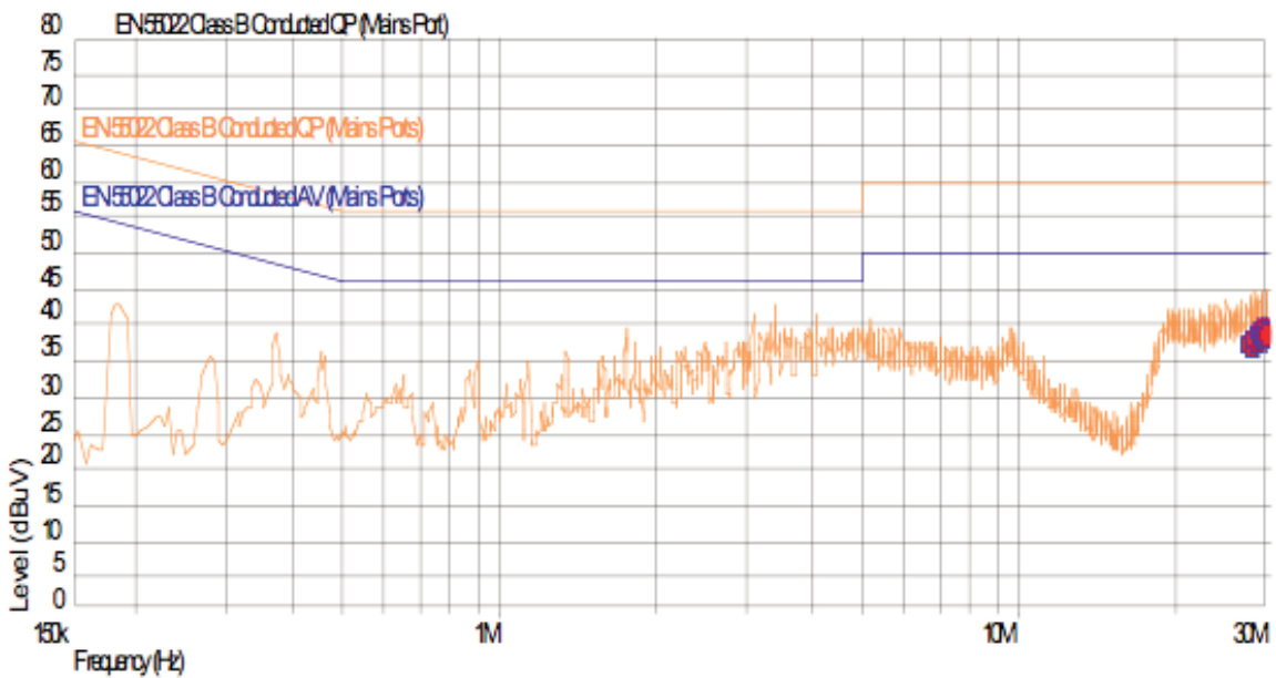
Figure 10 - QP Detector - LCL150PS12
