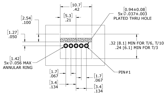
Figure 3. OKR Series Component locations are typical.
