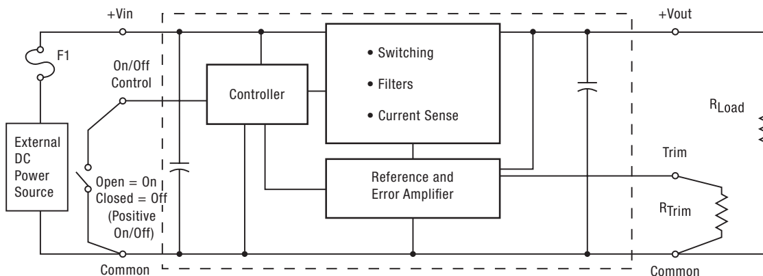
Figure 1. Connection Diagram
