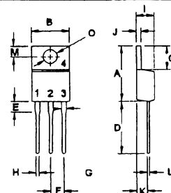
TO-220
