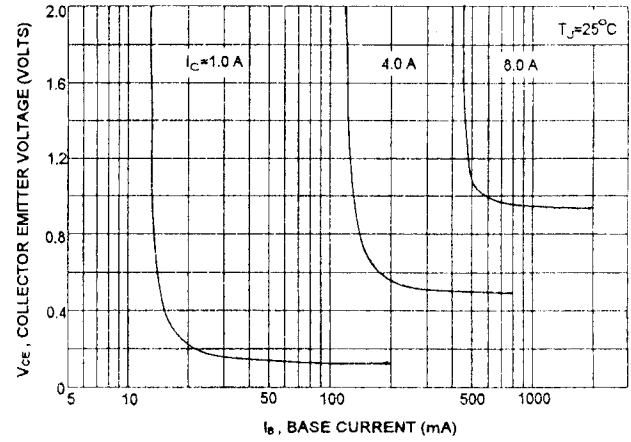
"ON" VOLTAGES
