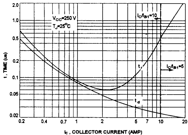
TURN-ON TIME
